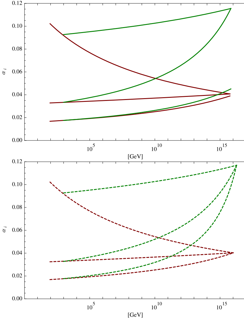
Fig. 3. Running of the gauge couplings is compared for \mathcal{F}\text{-}SU(5)_0 (solid red) vs. \mathcal{F}\text{-}SU(5)_I (solid green) and SU(5)_0 (dashed red) vs. SU(5)_I (dashed green). The upper line of each set depicts \alpha_3 , with \alpha_2 beneath, and then \alpha_Y . (For interpretation of the references to color in this figure, the reader is referred to the web version of this article.)
