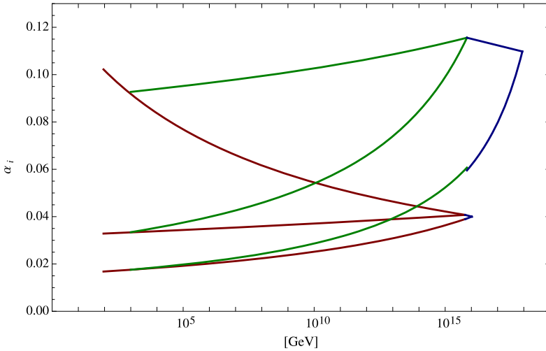
Fig. 7. In this plot we follow the Flipped SU(5) \times U(1)_X Type II model (solid green) further upward to a possible super unification (solid blue) just shy of 10^{18} [GeV]. This is nearly two orders of magnitude heavier than the corresponding extension of the Type 0 model (solid red) with MSSM content only. The running is computed to two loops. (For interpretation of the references to color in this figure, the reader is referred to the web version of this article.)
