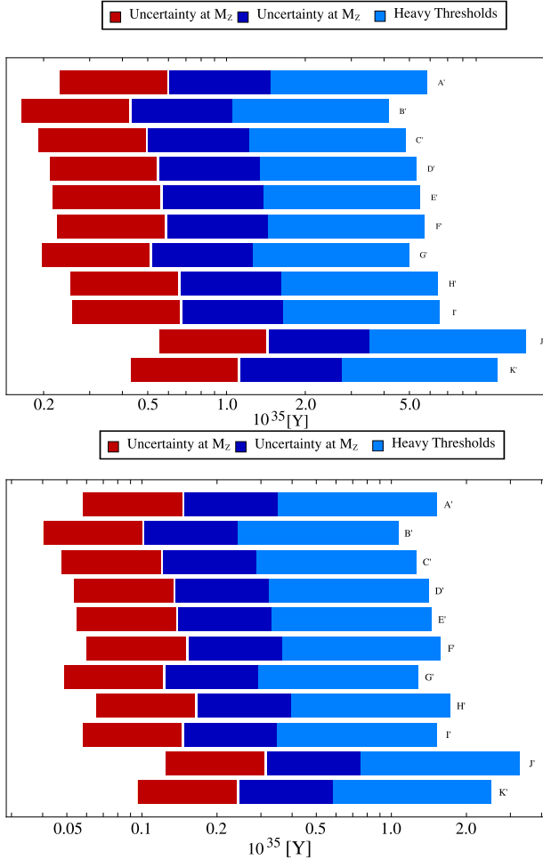
Fig. 6. The central value and key uncertainties of the predicted proton lifetime \tau_p^{(e|\mu)+\pi^0} are depicted for each of the benchmark scenarios (A'–K') for Flipped SU(5) with MSSM field content only (upper) and adding Type II vector-like multiplets (lower), respectively. The central prediction lies at the thin white line dividing the dark red and blue bands which themselves represent the cumulative uncertainty, combined in quadrature, in the electroweak mass scale M_Z and the coupling parameters ( \alpha_{em}, \sin^2 \theta_W^{\overline{MS}}, \alpha_s ) measured at that scale, cf. Eq. (46). The most significant variation is by far attributed to the strong coupling. The light blue bar represents plausible action of the unknown heavy thresholds as described in Sections 4.3, 5.3, measured from the central value, and acting only to slow decay in all cases. The second loop is computed once for each benchmark at the central evaluation point. The overall left to right motion of the bar sets gives some idea of the variation attributable to motion within the supersymmetric parameter space. It is a factor somewhat larger than two, comparable to the M_Z -scale uncertainties. Other potential sources of error, such as that from the hadronic matrix elements, are expected to be smaller in magnitude. (For interpretation of the references to color in this figure, the reader is referred to the web version of this article.)
