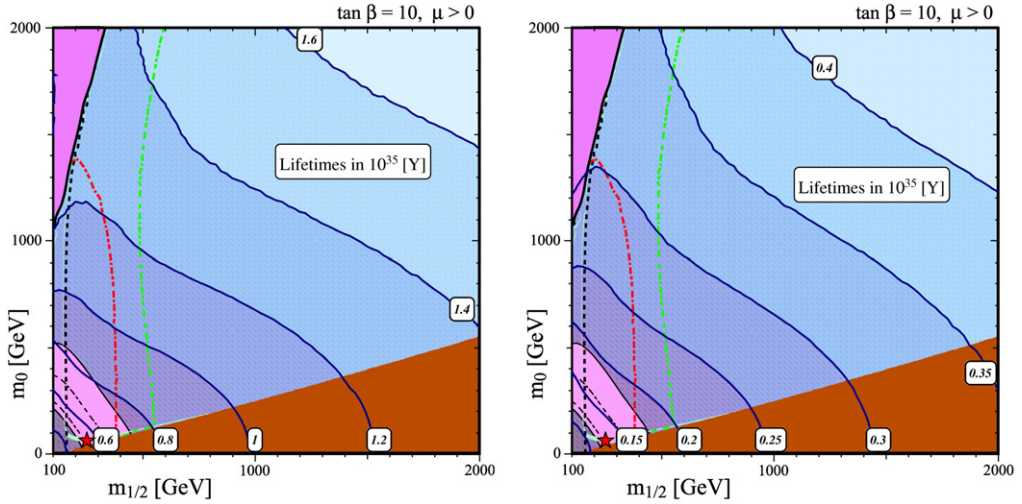
Fig. 5. Proton \tau_p^{(e|\mu)^+\pi^0} lifetime contours (dark blue), for Flipped SU(5) first with only MSSM field content, and subsequently including Type II vector-like multiplets, are overlaid onto a background map of phenomenological limits on the CMSSM for \tan\beta = 10 , and \mu > 0 , that courtesy of Olive et al. [68]. The orange-brown regions in the lower right of each graphic suffer a charged LSP, while the dark pink at upper left fail electroweak symmetry breaking. The dotted green, red and black lines mark the scalar neutralino–nucleon cross section at 10^{-9} [pB], the Higgs at 114 [GeV], and a chargino mass of 104 [GeV]. The light pink band in the lower left is consistent with measurements of (g-2)_\mu , and the narrow turquoise strip marks agreement between the cosmological CDM limits from WMAP and the relic neutralino prediction after coannihilation. Our baseline benchmark B' (red star) sits in the \mathcal{F} -ast lower left corner of each diagram. (For interpretation of the references to color in this figure, the reader is referred to the web version of this article.)
