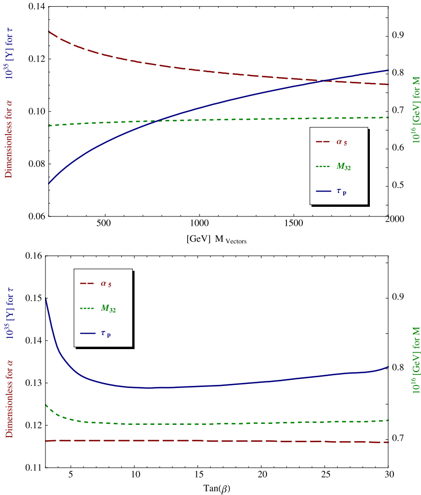
Fig. 4. The left-hand numerical scales here perform double duty, read dimensionlessly for \alpha_5 , and in units of [10^{35} \text{ Y}] for the proton partial lifetime \tau_p^{(e|\mu)+\pi^0} . M_{32} is read on the right-hand scale in [10^{16} \text{ GeV}] . The first example visually explores variation of these parameters with respect to changes in the mass of the F-theory vector-like multiplets of Flipped SU(5) Type II. The vector mass is run from 200 [GeV] up to 2 [TeV], bookending the value of 1 [TeV] to which we otherwise default. The SUSY spectrum is taken at benchmark B' as usual. We see a decline in the coupling strength as the vector mass increases, with the (partial) unification mass holding essentially steady. The result is a modest gradual rise in proton lifetime from left to right, starting some 25% below, and ending some 15% above our baseline value. In the second plot we instead vary the SUSY Higgs parameter \tan\beta from 3 to 30, bounding again our default value of 10 for benchmark B' . We regenerate the SUSY spectrum along this span with ISASUGRA, otherwise leaving the B' input parameters intact. This change of approach with respect to the spectrum is responsible for some overall up-tick in the lifetime. The model again is Flipped SU(5) Type II, with the vector mass locked at 1 [TeV]. In this example we instead see \alpha_5 flatline, while the unification mass declines steeply to a minimum near our default region, thereafter rebounding slowly. The proton lifetime tracks with and amplifies changes in the unification mass, although the overall variation is still mild, the peak within about 15% of the valley for the range considered. The slope approaching the left edge however is steep, and continuing too far outside the graph in either direction we experience pathologies in application of the Yukawa boundary condition for calculation of the second loop.
